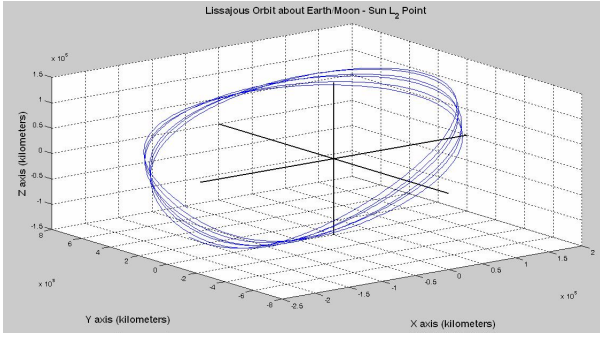
Figure 4. Leader (Telescope) Spacecraft Trajectory about Earth/Moon-Sun L_2 point
