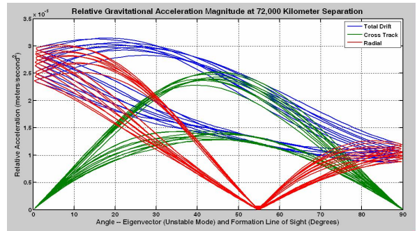
Figure 7. Relative Acceleration of Follower with Respect to Leader for Observation Vector within the Ecliptic Plane as a Function of Angular Separation Between Observation Vector and eigenvector e_1 of {}^I\Xi(t_0) .
