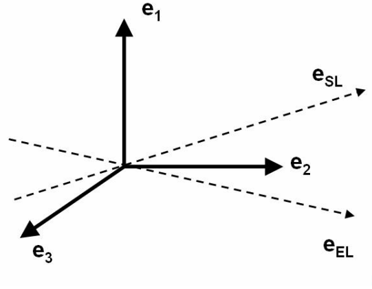
Figure 3. Orientation of Eigenvectors ( \mathbf{e}_1 , \mathbf{e}_2 , \mathbf{e}_3 ) of {}^I \Xi(t_0) relative to \mathbf{e}_{SL}(t_0) and \mathbf{e}_{EL}(t_0)
