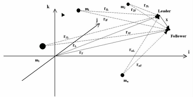
Figure 2. Two Spacecraft Under the Gravitational Influence of n-Bodies
